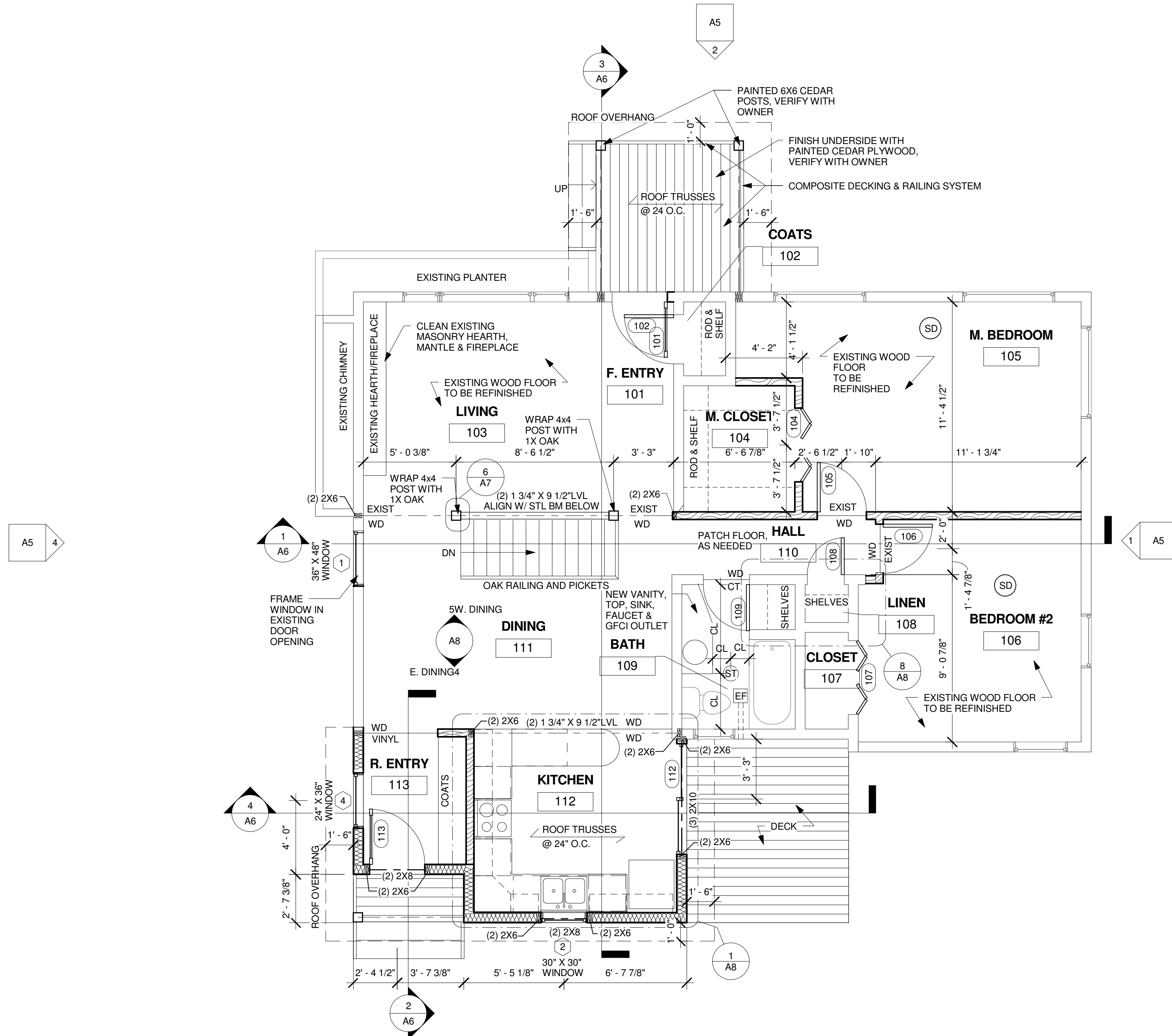
① MAIN LEVEL 1/4" = 1'-0"
