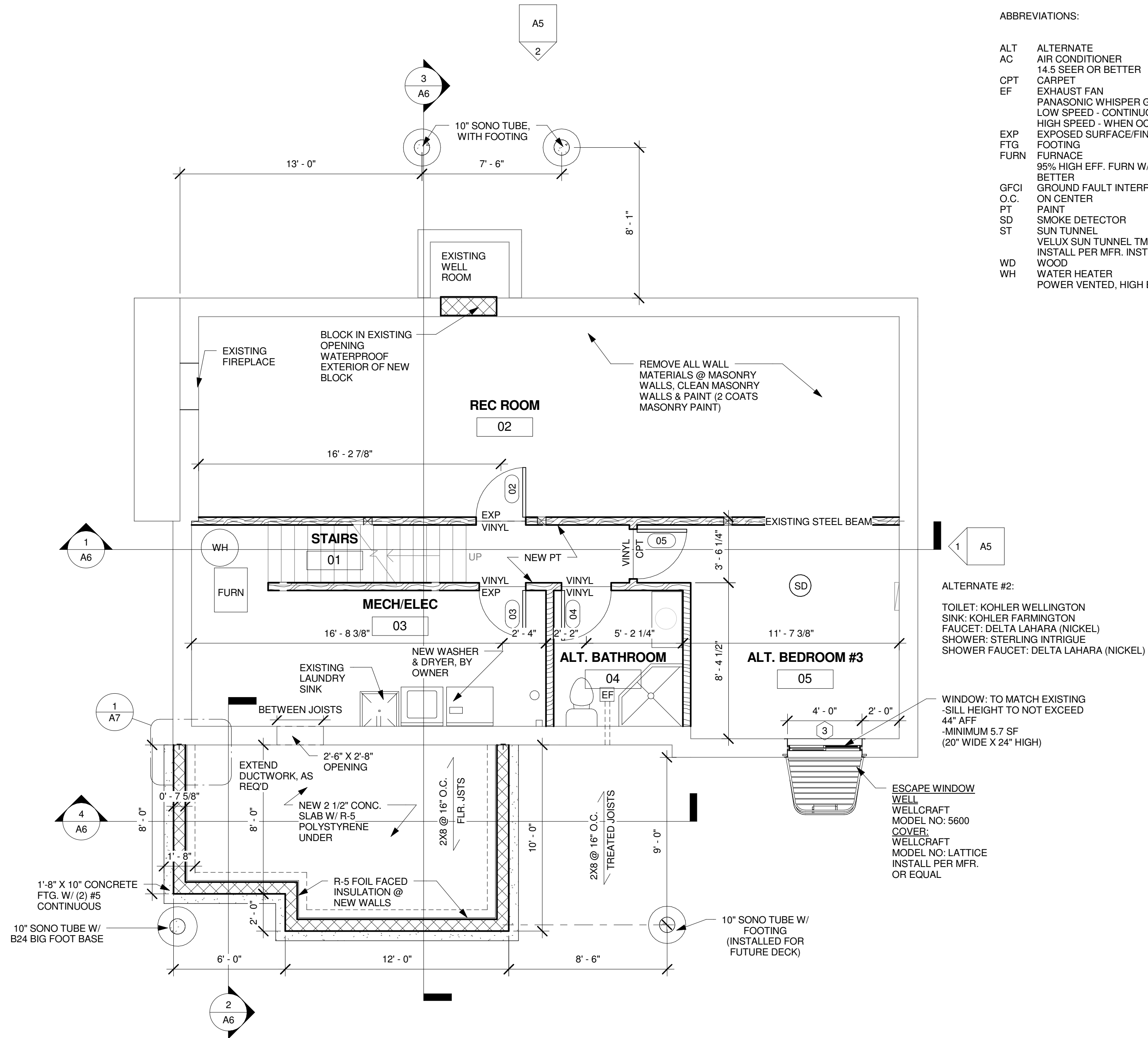
1 LOWER LEVEL 1/4" = 1'-0"
